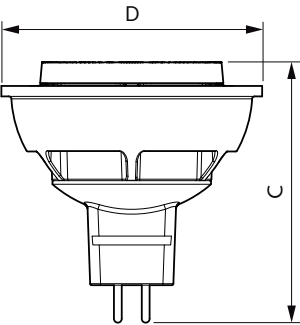
MR16 6.5-25W 410lm 25D Dimtone GU5.3 D
